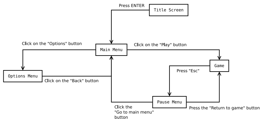
Figure 323: Diagram of a menu system’s state machine
